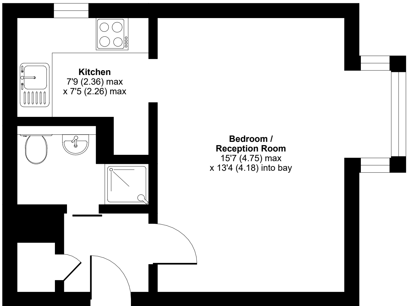
GROUND FLOOR
